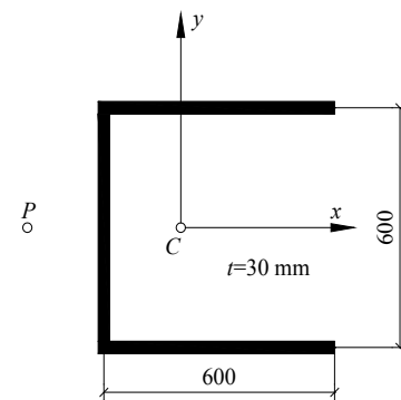
Figure 2 Cross section layout for Example 2
