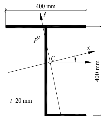
Figure 3 Cross section layout for Example 2
